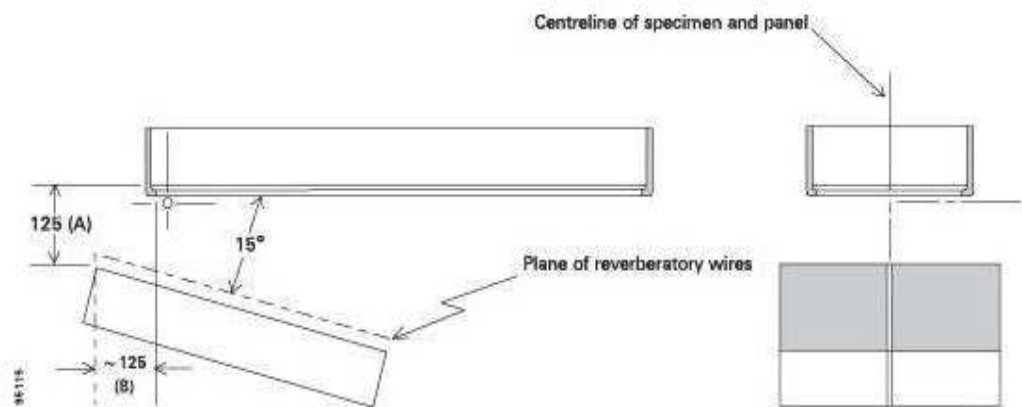
Figure 3 – Specimen – panel arrangement
