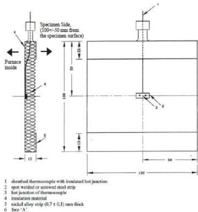
Figure 4 – Furnace thermocouple assembly
