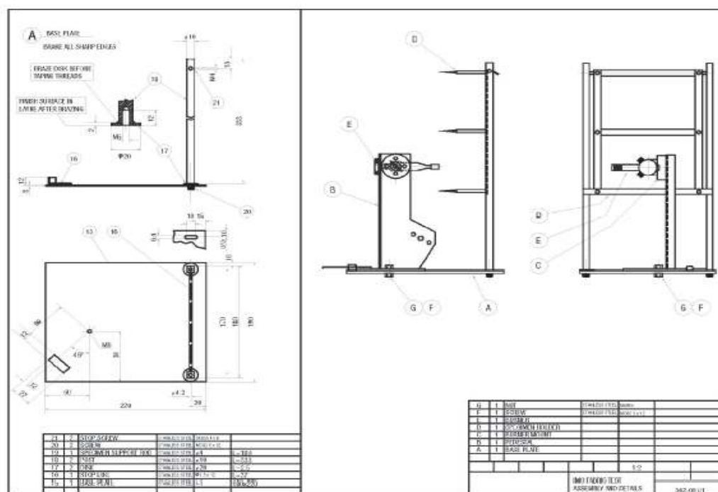
Figure 3 – Fabric test assembly and details
