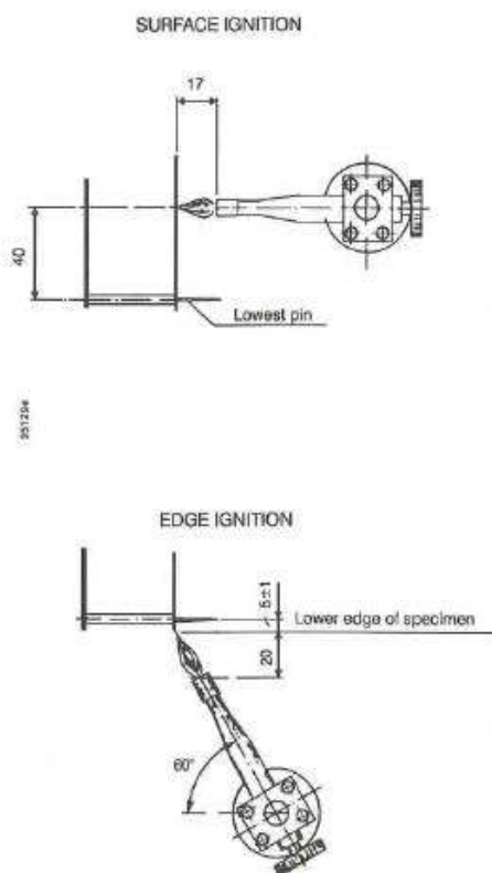
Figure 2 – Ignition burner: fabric positions
