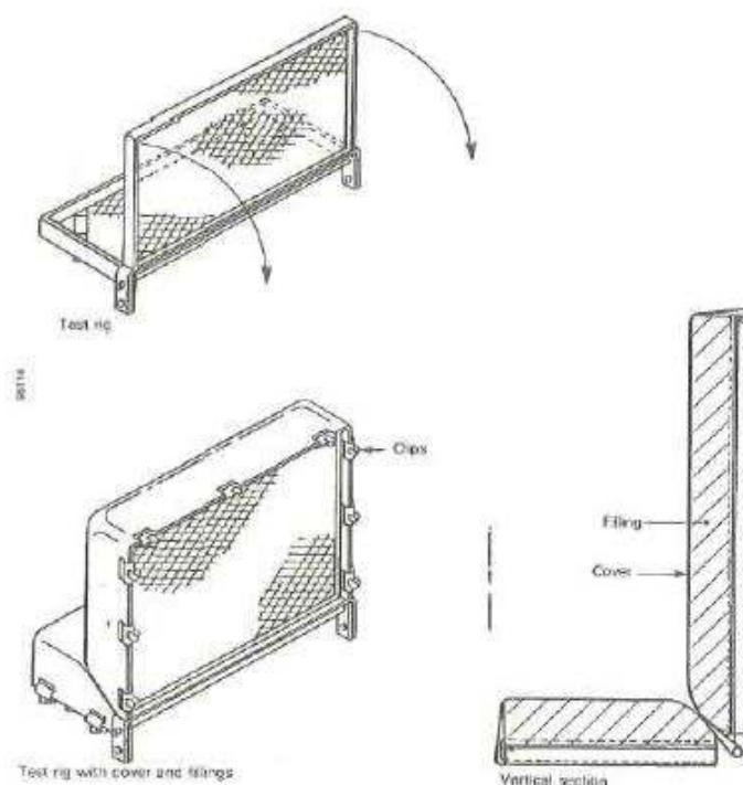
Figure 2 – Test rig assembly
