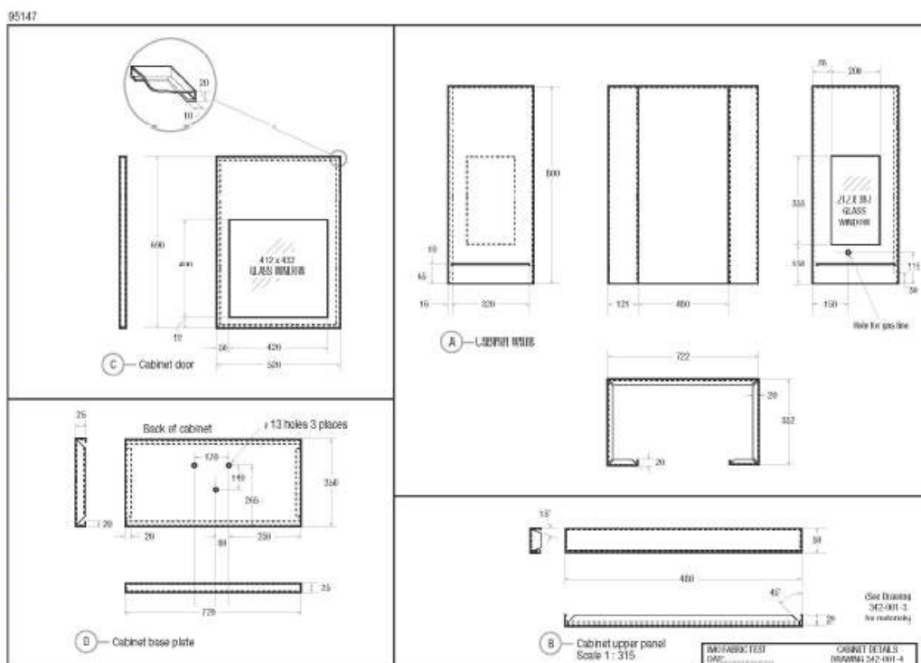
Figure 6 – Fabric test: test enclosure
