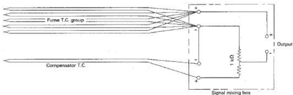
Figure 7 – Diagrammatic sketch of thermocouple circuit
