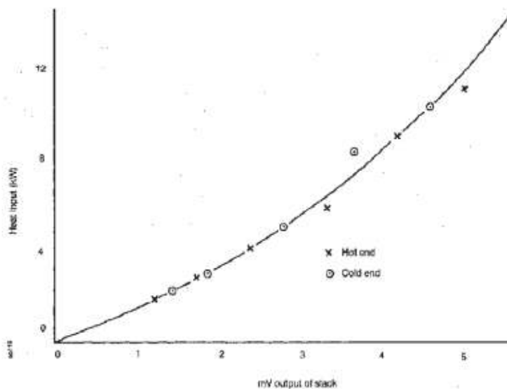
Figure 9 – Example of a typical stack calibration
