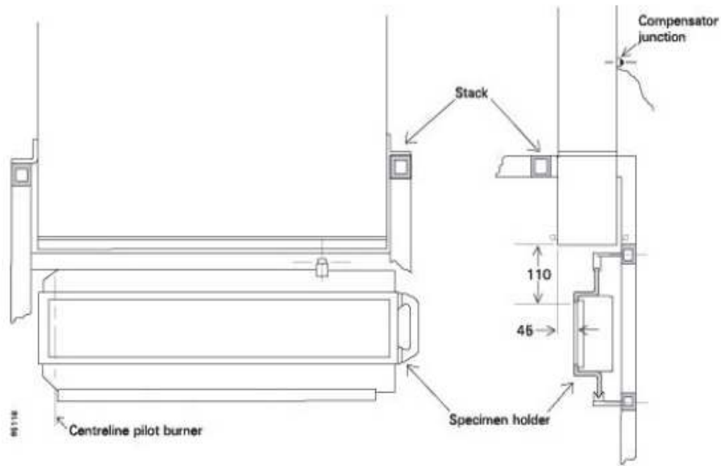
Figure 4 – Position of stack and specimen
