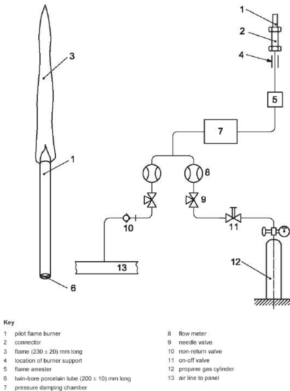
Figure 5 – Pilot burner details and connections
