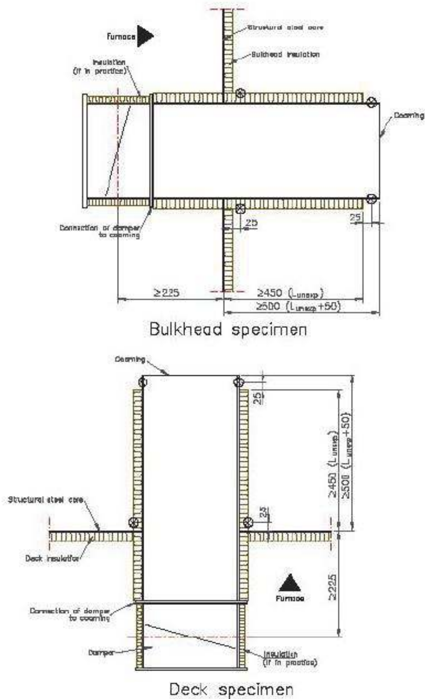
Figure A1 – Fire dampers: insulation on test specimens and position of unexposed-face thermocouples
