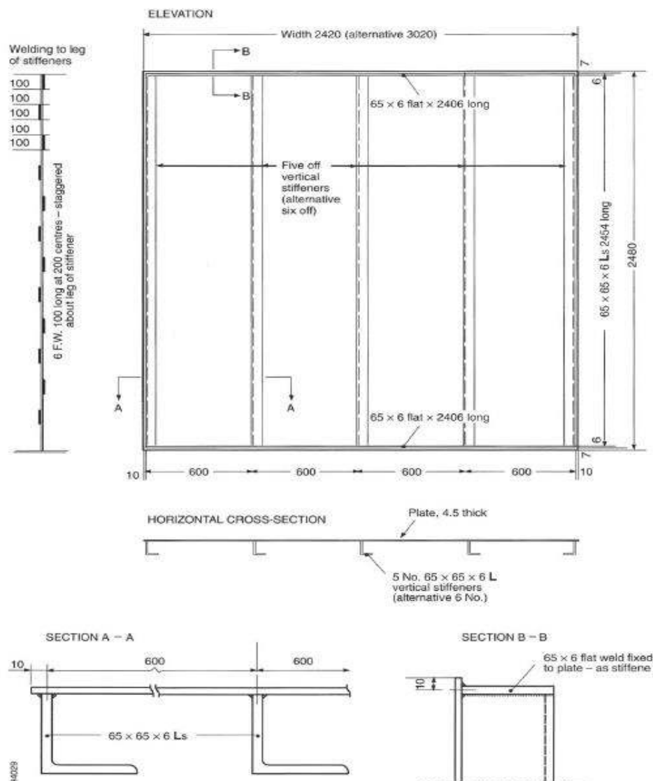
Figure 1 – Structural steel core for "A" class bulkhead and "B" class lining
