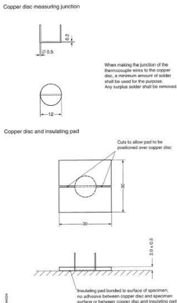
Figure 6 – Unexposed-surface thermocouple junction and insulating pad
