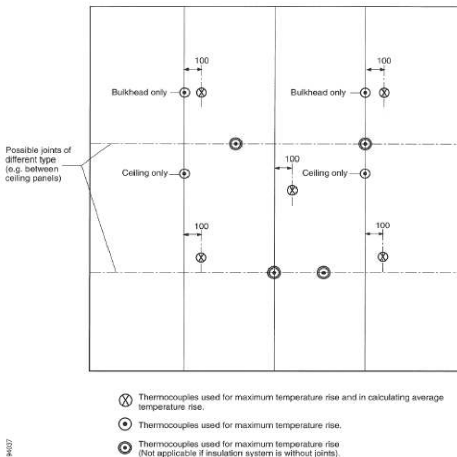
Figure 9 – Position of unexposed-face thermocouples for "B" and "F" class divisions
