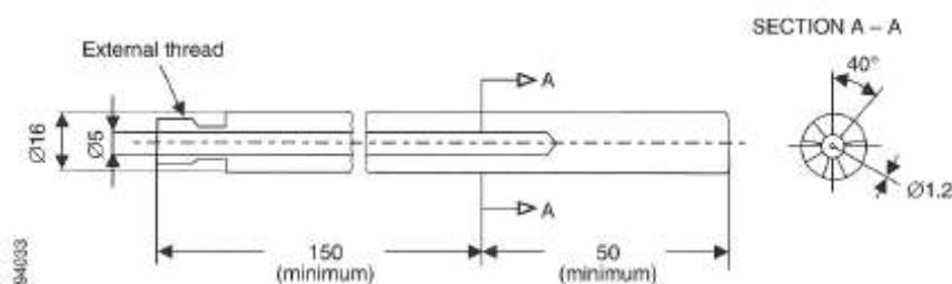
Figure 5 – Pressure-sensing heads
