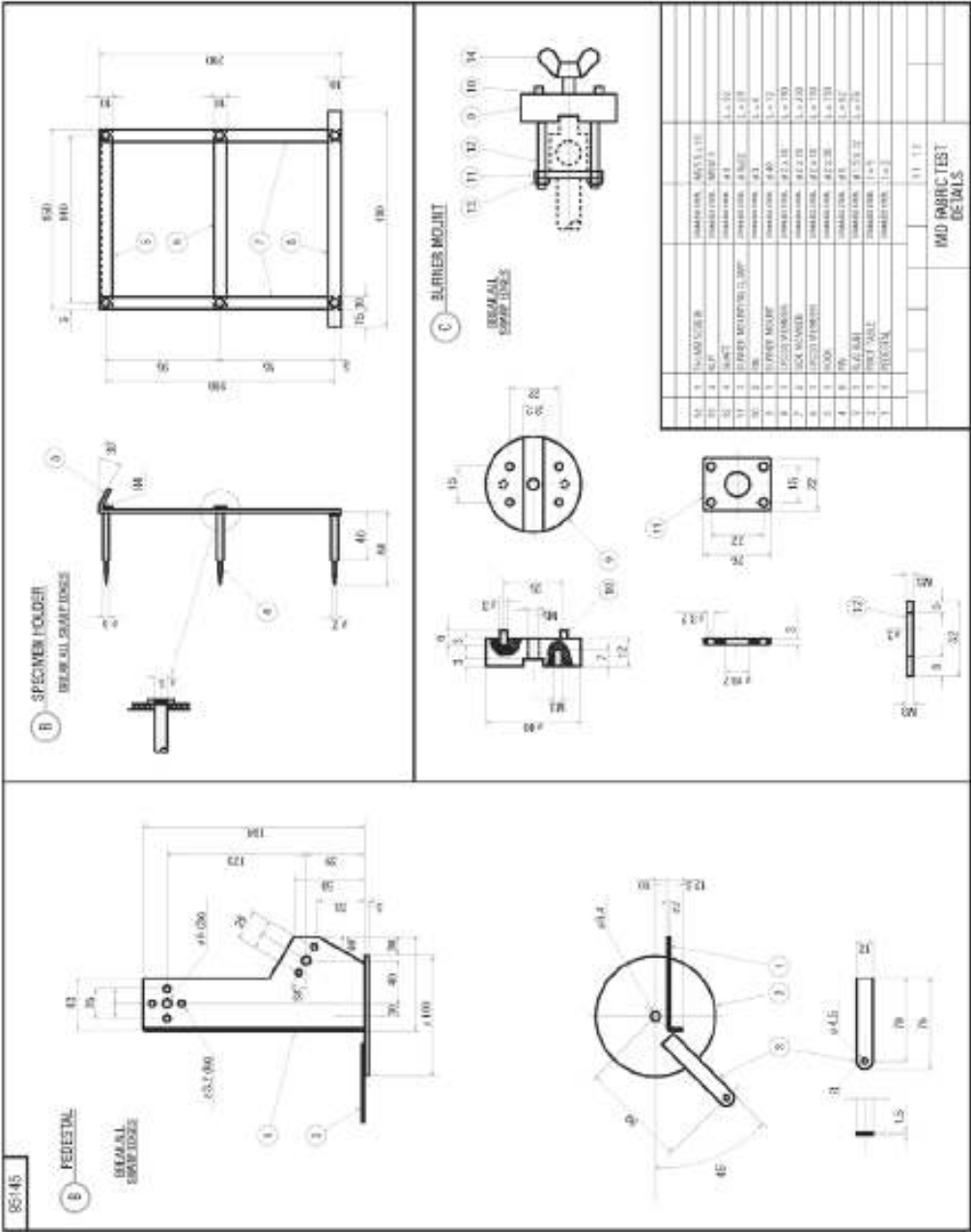
Figure 4 – Fabric test: details
