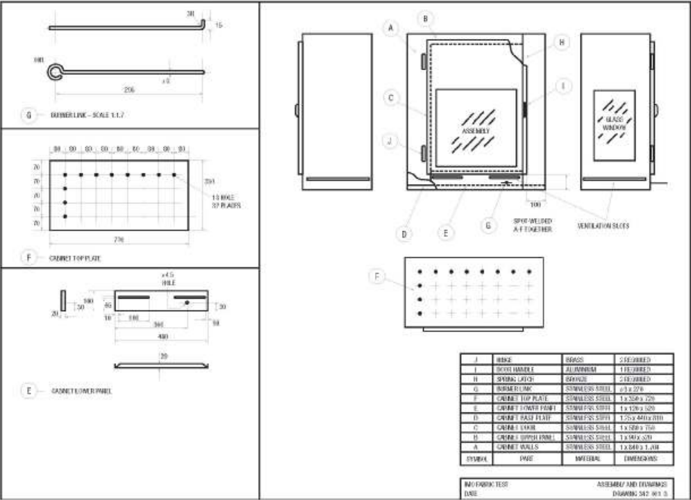
Figure 5 – Fabric test: test enclosure
