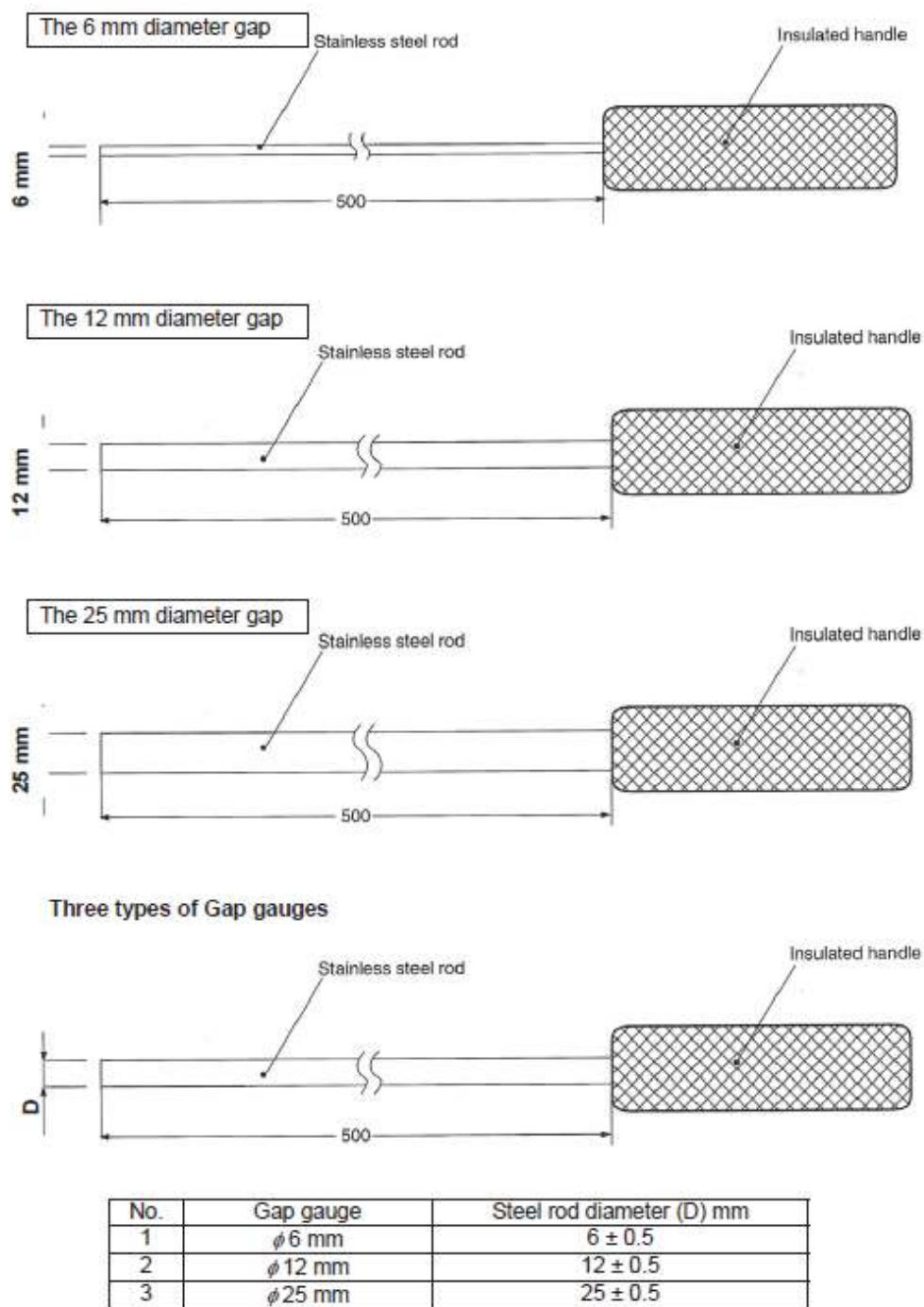
Figure 11 – Gap gauges
