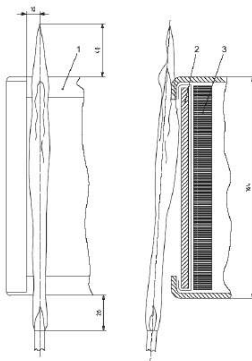
Figure 6 – Position of pilot flame
