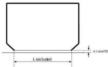
Prismatic tanks
