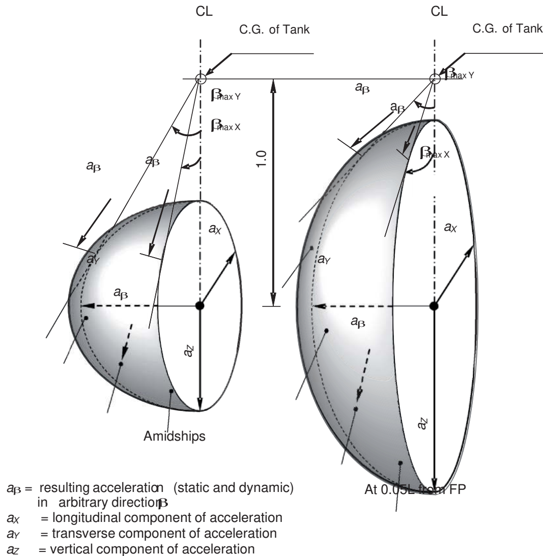
Figure 4.1 – Acceleration ellipsoid
