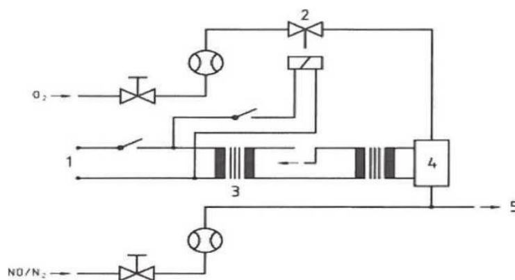
Figure 1 - Schematic representation of NOi converter efficiency device
