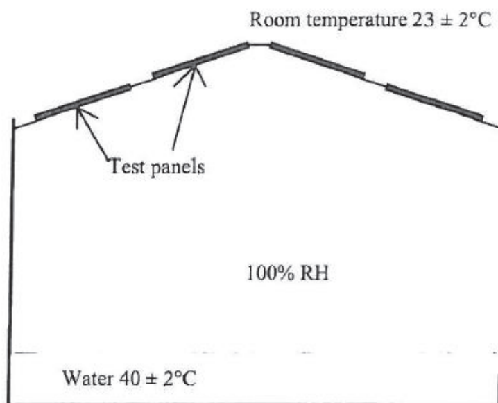
Figure 2 Condensation chamber
